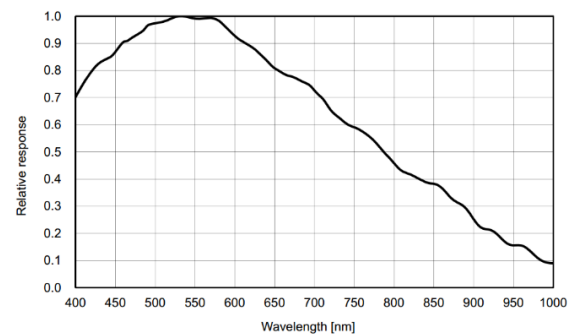
MV-CE200-10GM Quantum Efficiency
