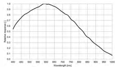
MV-CH310-10XM-F-NF
