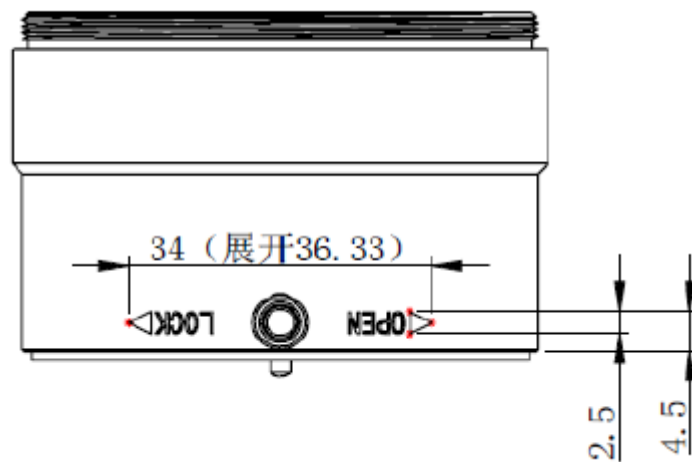
镜头转接环 M58x0.75-F T35
